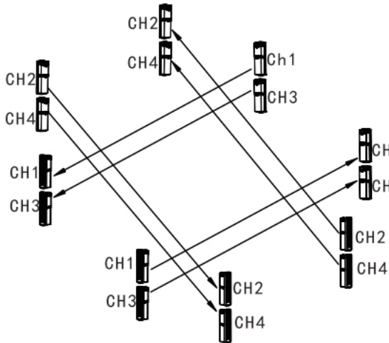
(3) Perimeter installation 1
